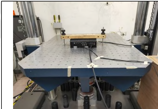
13. Mechanical Shock Test: -Z axis
